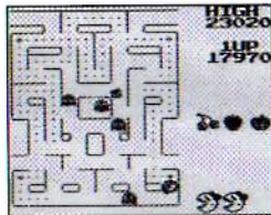
1/2 Maze
